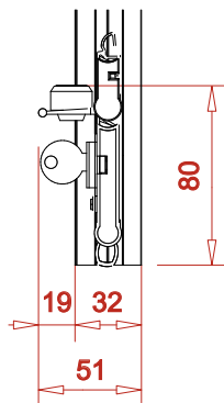
PPC side view
